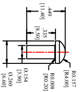
Type "A" Ø4,0mm Plain Rivet
